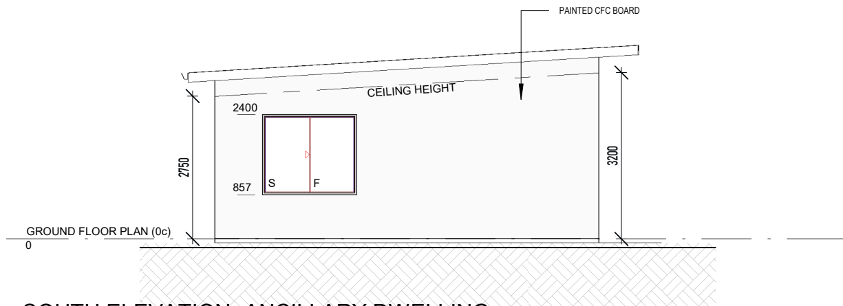
SOUTH ELEVATION- ANCILLARY DWELLING 1 : 100
