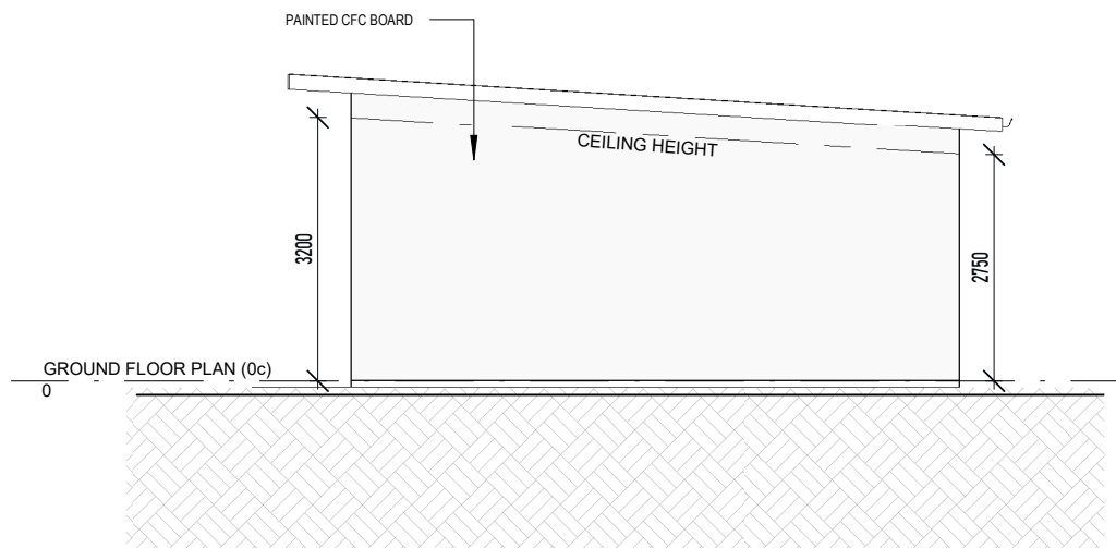
NORTH ELEVATION- ANCILLARY DWELLING 1 : 100
