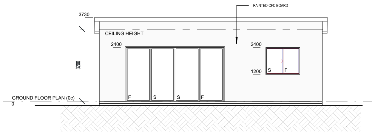
EAST ELEVATION- ANCILLARY DWELLING 1 : 100
