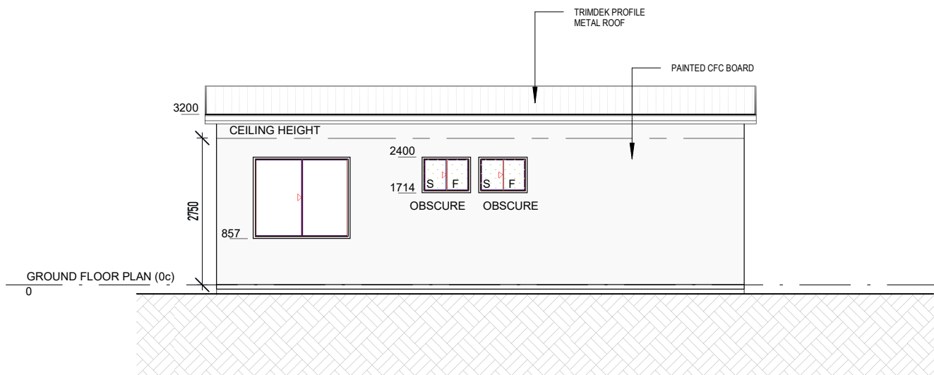
WEST ELEVATION- ANCILLARY DWELLING 1 : 100
